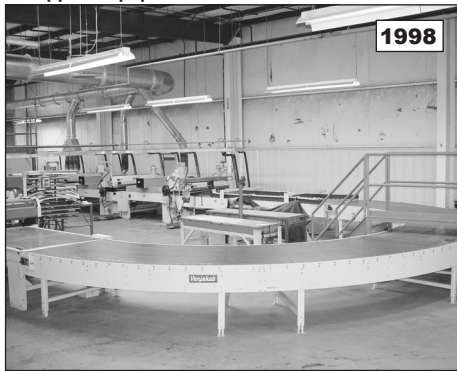
Venjakob 180° Turn Belt Conveyor
