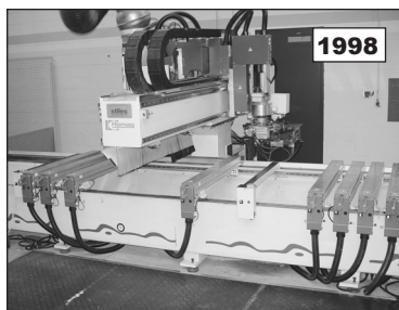
Homag BAZ 32 K (CNC) Router & Edgebander Machining Center
