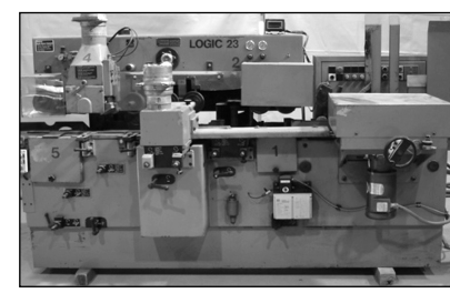
SCMI Logic 23 Moulder
