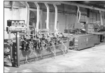
Late Model Kval Door Machinery (3) Lines Available!
