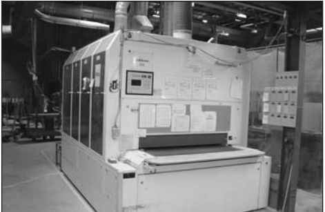
Heesemann 53" Crossbelt/Widebelt Sander
