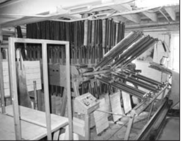
Taylor & Doucet 40 Section Auto. Clamp Carrier
