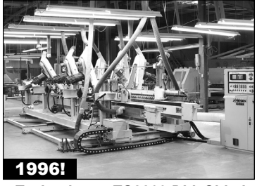
1996! Technolegno TG2800 Dbl. Sided Profile Shaper/Sander
