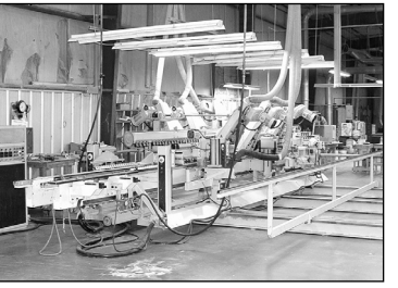
Technolegno Dbl. Sided Profile Shaper/Sander
