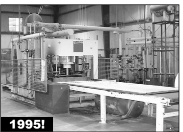
1995! Wemhoner KT-M34/15V-300 Shuttle Style Membrane Hot Press & Boiler
