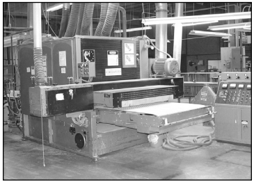
Timesaver 852.4CB 3-Head Wide Belt Cross Belt Sander W/Sensing
