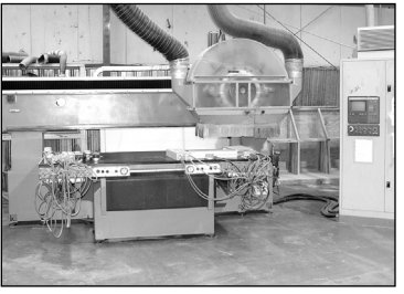
CMS NC-TRIAX-PF-1.R8RR Single Table CNC Router
