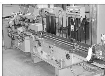
Weinig U22N 7-Head Feed Thru Moulder w/ Universal & Hopper Feed
