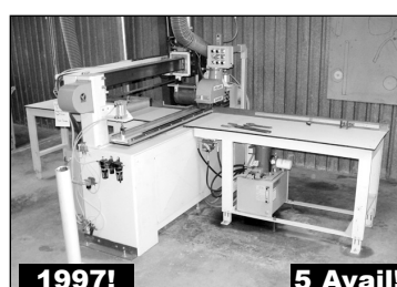
A & S Machinery V-Groover New in 1997!
