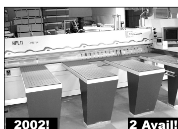
Holzma Optimat HPL11/43/16 Rear Load CNC Panel Saw New in 2002! (2) Available!
