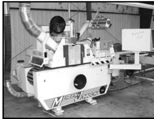
Mereen Johnson 312-DC/SR Dip Chain Multiple "Select-A-Rip" System w/ Feeding Table (new in 2001)
