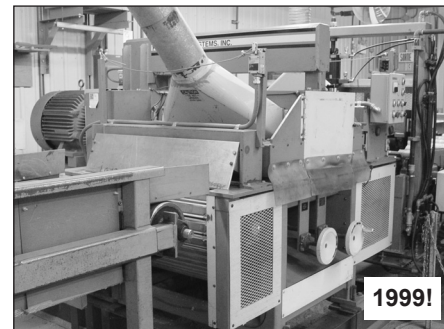
Progressive SB/D-31 31" Gang Rip
