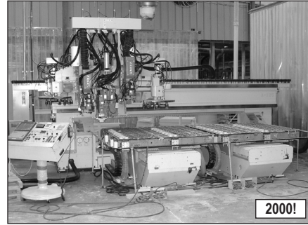
Shoda Super Max Twin Table CNC Router
