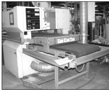
Timesaver Top & Bottom Planer Sander Line
