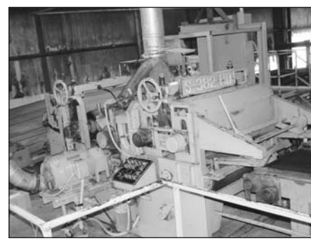
Newman S-382 Planer
