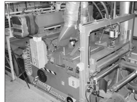
Merein Johnson 424 DC/SR Gang Rip Saw & Group 7 Overhead Scanner & Fence
