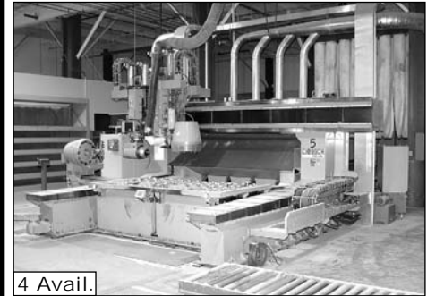
Heian NG-251-MC CNC Routers w/ Tool Changers (4 Axis)
