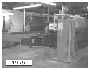
Fletcher FM-210 tilting cut off, tilt tenon, tilt high speed jump cope, tilt high speed cope
