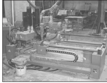
Friulmac FN7 Hopper Feed T & B Tenon, Cope (works well in front of moulder)
