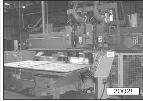
Heian CNC Router HR-242PMC-1616W (2) Routers w/ (2) 12 position Tool Changers
