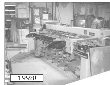
Vitap Sigma 2TA Feed Through 32mm Borer
