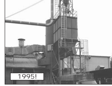
Torit 376RFW-10 (1995) Bag House 75HP Blower, rotary air lock
