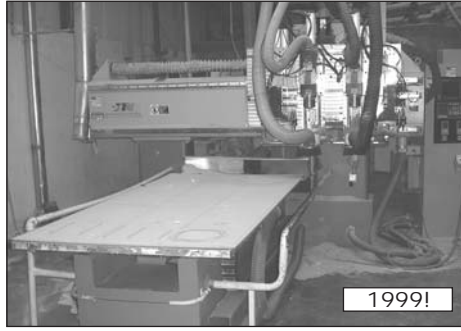
Northwood NW-48 CNC (2) Routers w/ (2) 8 position Tool Changers
