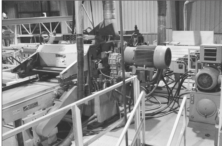
Newman Whitney S382 Planing Line w/ Break Down Tilt Hoist, Desticker, Grading Drop Out, & Jouliau Vacuum Stacker
